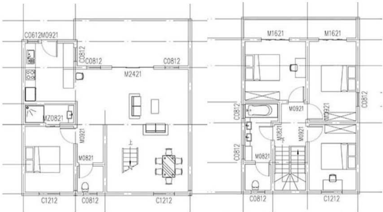
First floor
