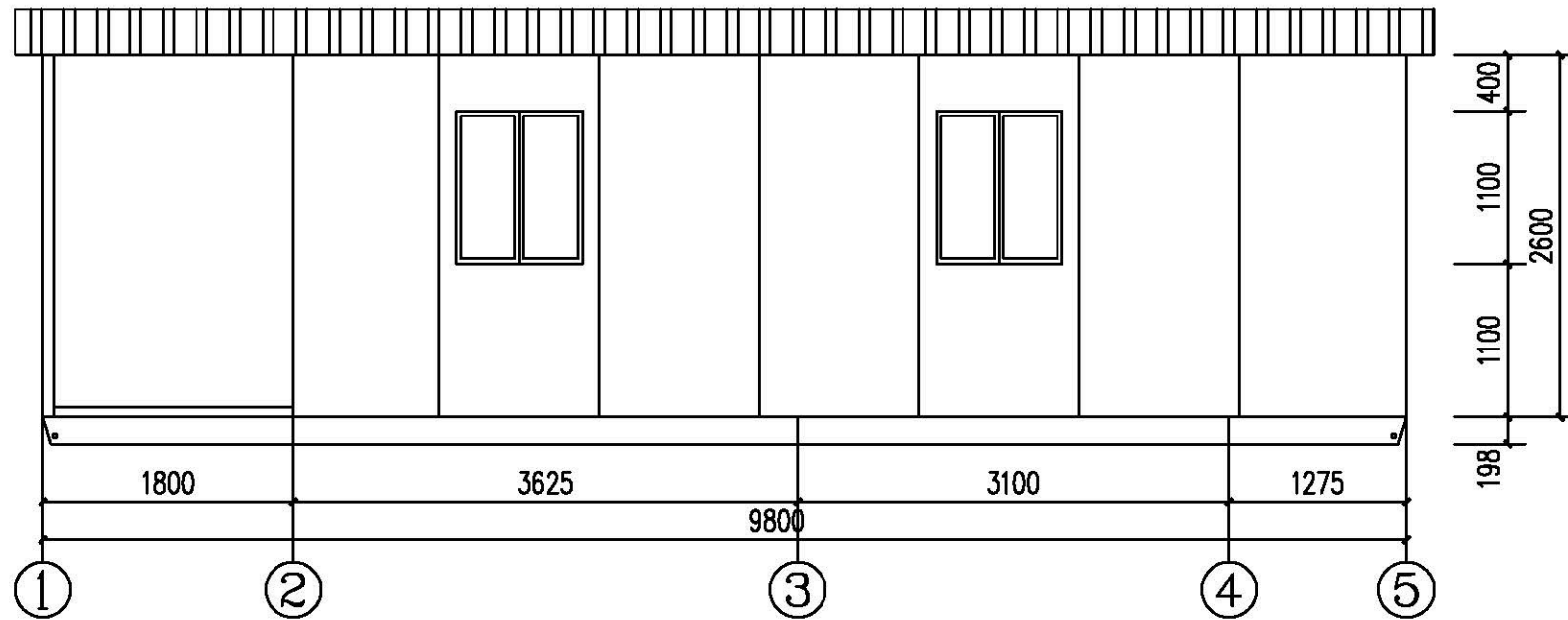
AXES ELEVATION A
