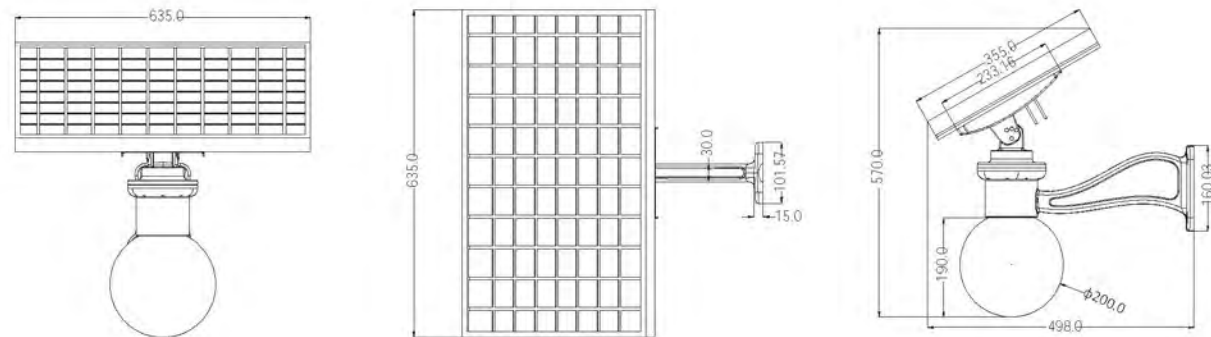
BS-ML-12 dimension
