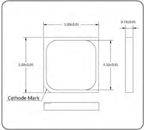
LED Chip Dimension
