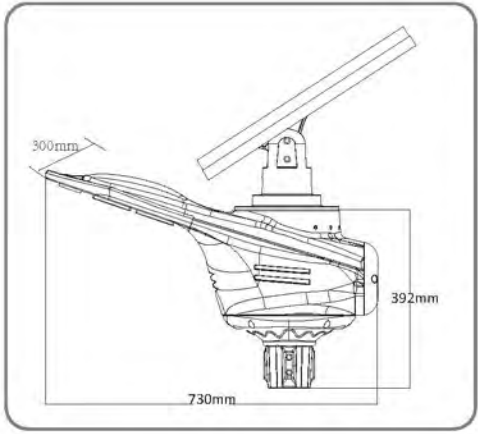
Lamp Dimension
