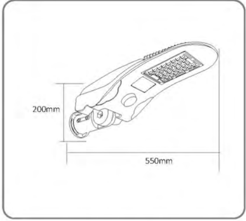
Lamp Dimension
