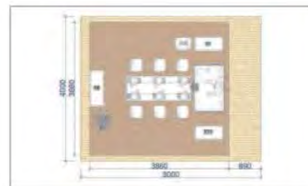
Interior Plan of Small A Tent 小A帐篷室内平面图
