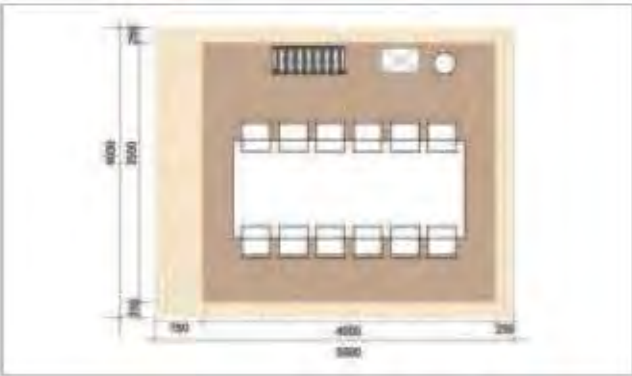
U4mini Restaurant Tent Interior Plan U4mini餐厅帐篷 室内平面图
