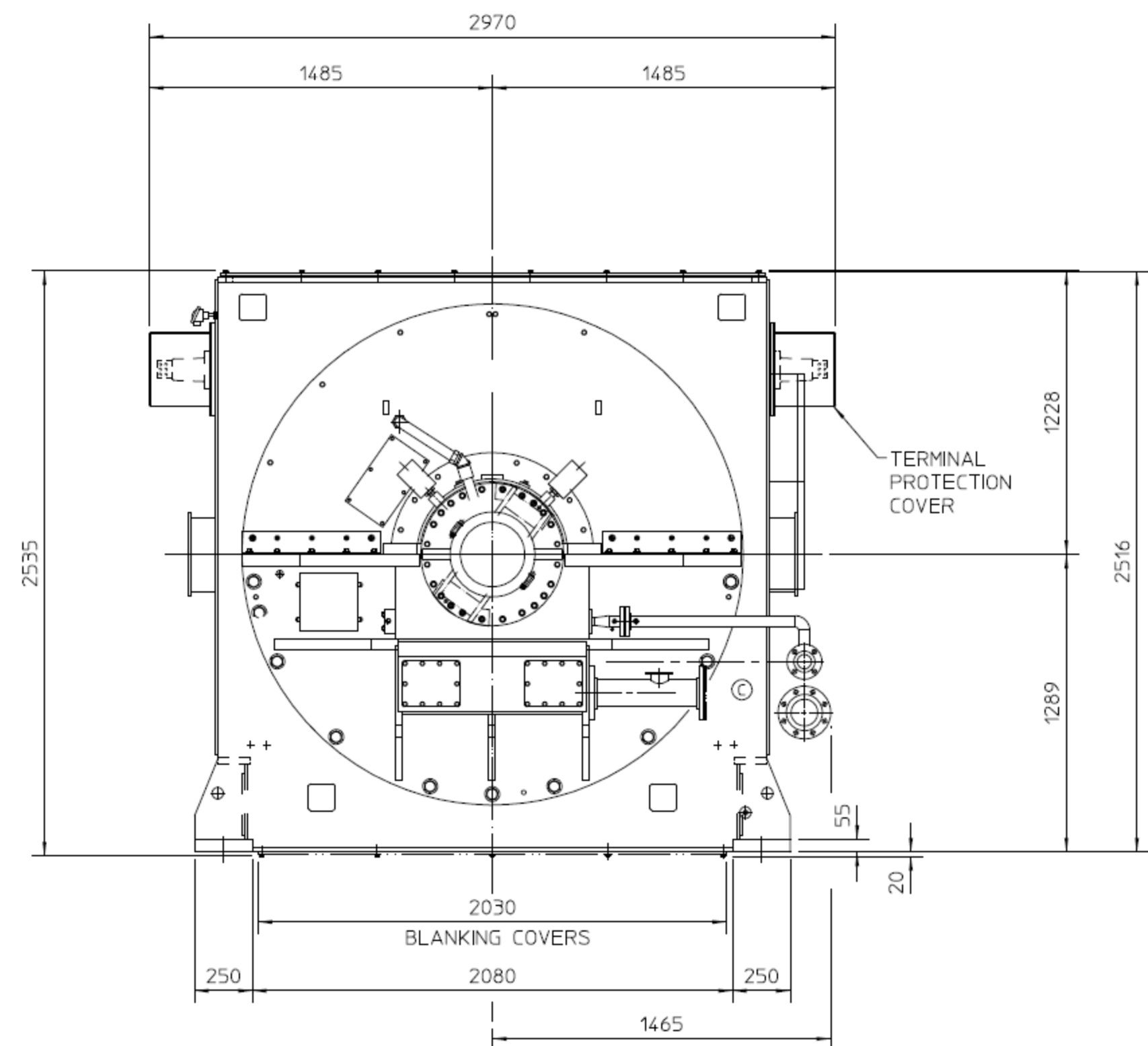
VIEW ON NON EXCITER (DRIVE) END
