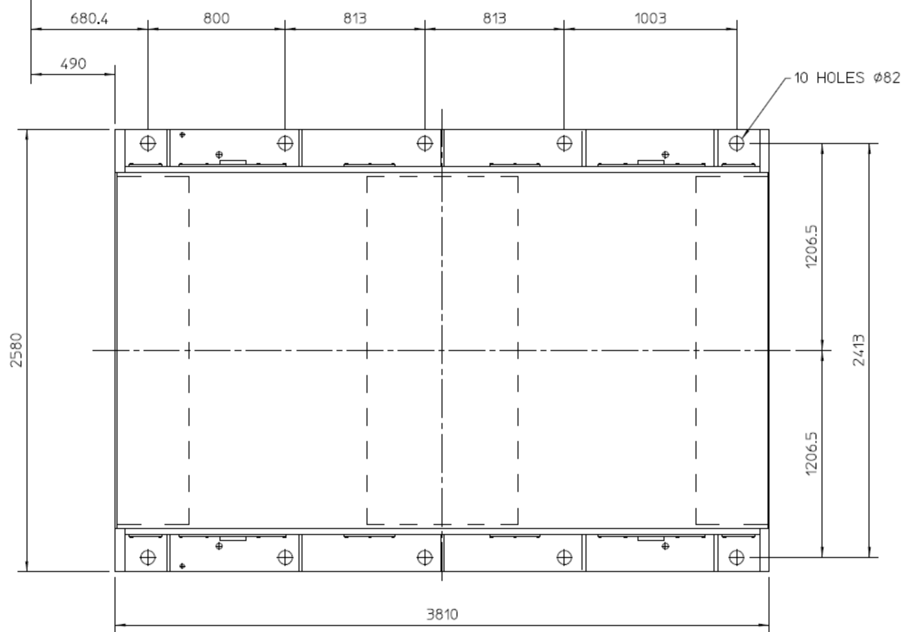
PLAN VIEW ON STATOR FEET
